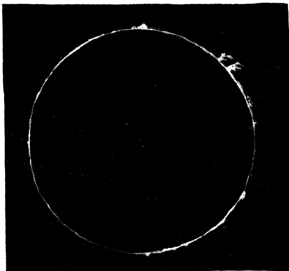
THE CHROMOSPHERE AND PROTUBERANCES ( Photographed by Professor HALE, 25th July 1892, without an Eclipse )
